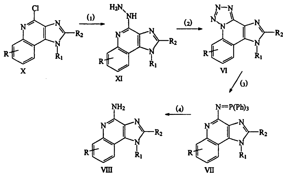
Reaction Scheme III
